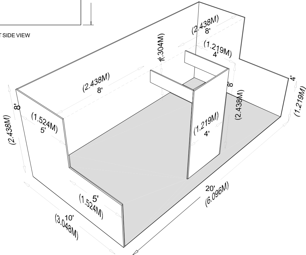
10' X 20' CLOTH/DRAPE PERIMETER BOOTH
